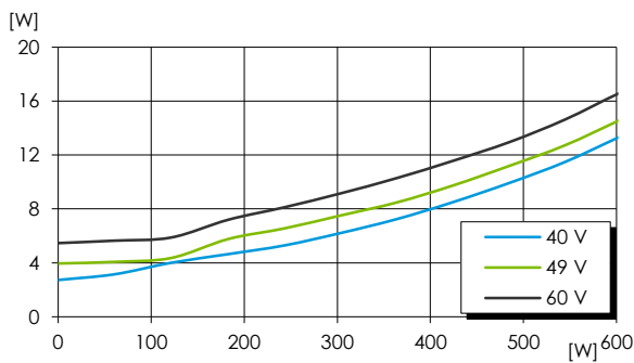
Dissipated power vs. output power and input voltage at T_{PI} = +90^\circ
