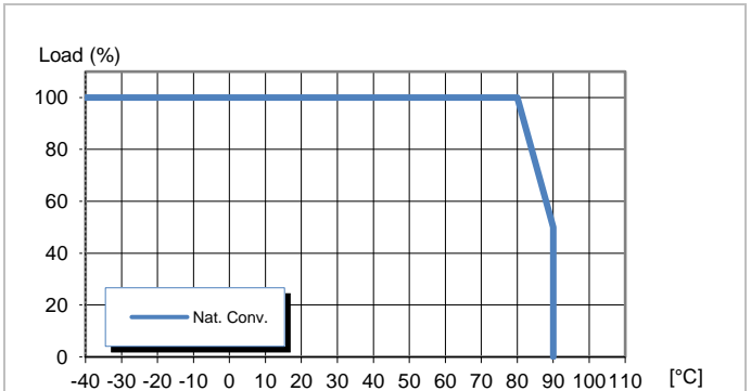
Available load vs. ambient air temperature. See Thermal Consideration section. (PUC1212S2B and PUC1212D2B)
