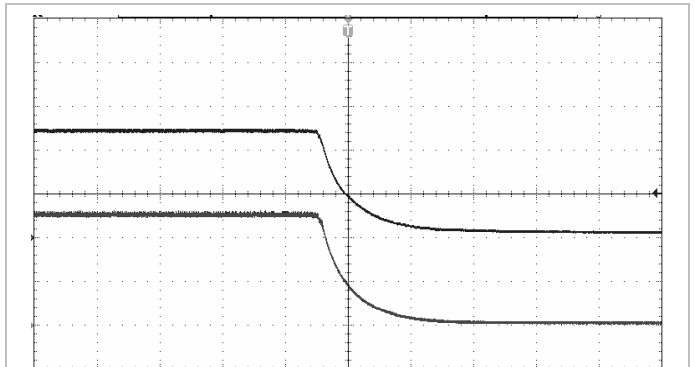
Shut-down, closed by disconnecting V_I at: T_{P1} = +25^\circ\text{C} , V_I = 24\text{ V} , V_O = 5\text{ V} I_O = 400\text{ mA} resistive load.
