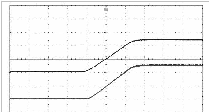
Start-up, enabled by connecting V_I at: T_{P1} = +25^\circ\text{C} , V_I = 24\text{ V} , V_O = 5\text{ V} I_O = 400\text{ mA} resistive load.
