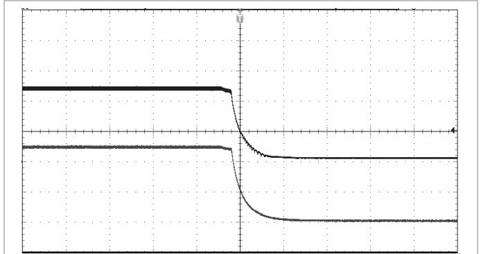
Shut-down, closed by disconnecting V_I at: T_{P1} = +25^\circ\text{C} , V_I = 12\text{ V} , V_O = 5\text{ V} I_O = 400\text{ mA} resistive load.
