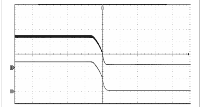
Start-up, enabled by connecting V_I at: T_{P1} = +25^{\circ}\text{C} , V_I = 5\text{ V} , V_O = 5\text{ V} I_O = 200\text{ mA} resistive load.
