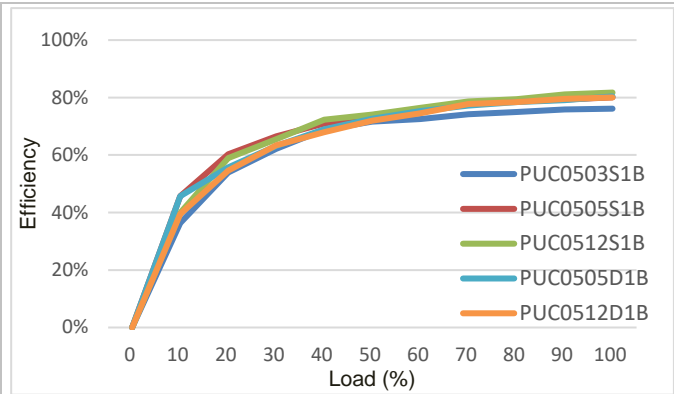
PUC05-1B Efficiency vs. load current at T_{P1} = +25^{\circ}\text{C} .
