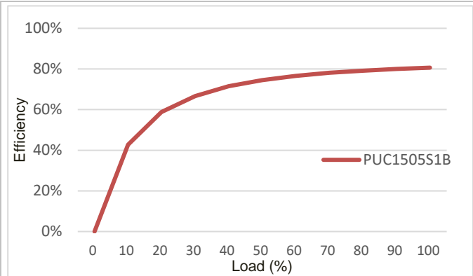
PUC15-1B Efficiency vs. load current at T_{P1} = +25^{\circ}\text{C} .
