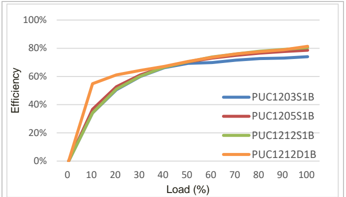
PUC12-1B Efficiency vs. load current at T_{P1} = +25^{\circ}\text{C} .
