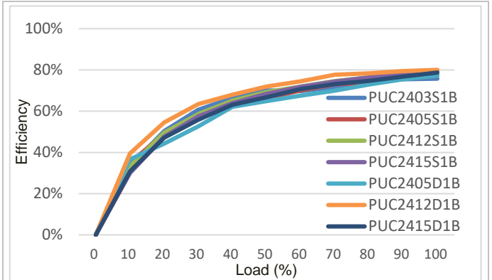
PUC24-1B Efficiency vs. load current at T_{P1} = +25^{\circ}\text{C} .
