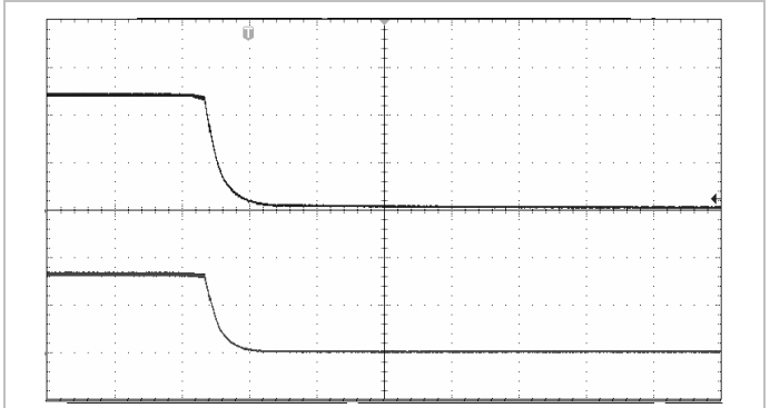
Shut-down, closed by disconnecting V_I at: T_{P1} = +25^\circ\text{C} , V_I = 24\text{ V} , V_O = 3.3\text{ V} I_O = 606\text{ mA} resistive load.
