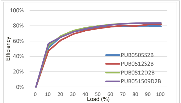
PUB05-2B Efficiency vs. load current at T_{P1} = +25^{\circ}\text{C} .
