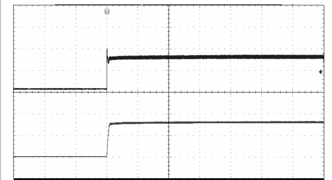
Start-up, enabled by connecting V_I at: T_{P1} = +25^\circ\text{C} , V_I = 3.3\text{ V} , V_O = 3.3\text{ V} I_O = 606\text{ mA} resistive load.
