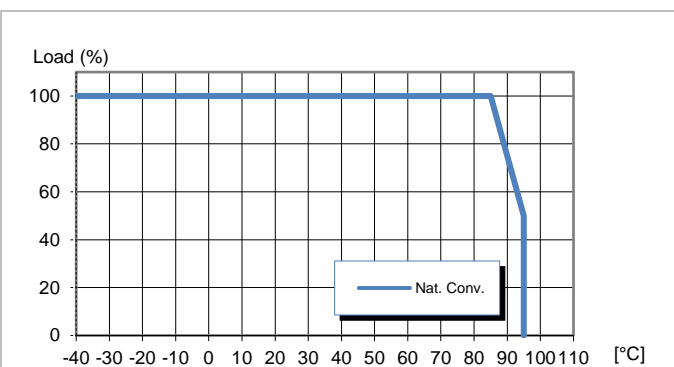
Available load vs. ambient air temperature. See Thermal Consideration section.
