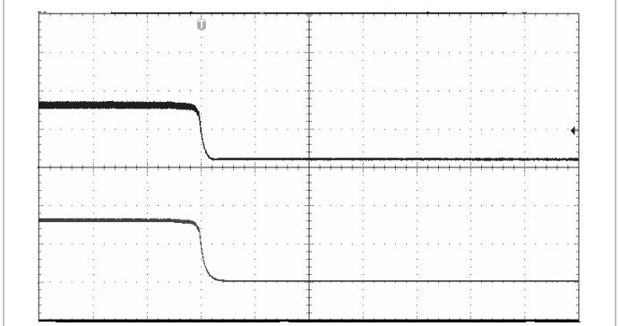
Start-up, enabled by connecting V_I at: T_{P1} = +25^\circ\text{C} , V_I = 3.3\text{ V} , V_O = 3.3\text{ V} I_O = 606\text{ mA} resistive load.
