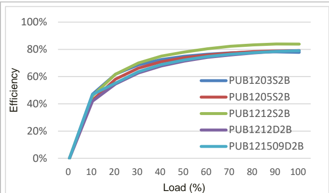
PUB12-2B Efficiency vs. load current at T_{P1} = +25^{\circ}\text{C} .
