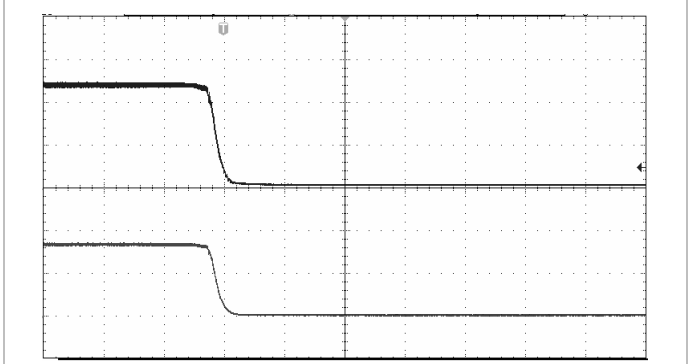
Shut-down, closed by disconnecting V_I at: T_{P1} = +25^\circ\text{C} , V_I = 12\text{ V} , V_O = 3.3\text{ V} I_O = 600\text{ mA} resistive load.
