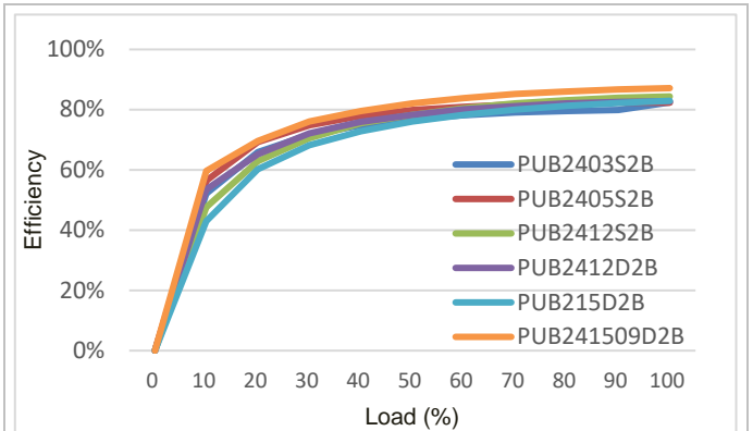
PUB24-2B Efficiency vs. load current at T_{P1} = +25^{\circ}\text{C} .
