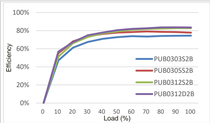
PUB03-2B Efficiency vs. load current at T_{P1} = +25^{\circ}\text{C} .
