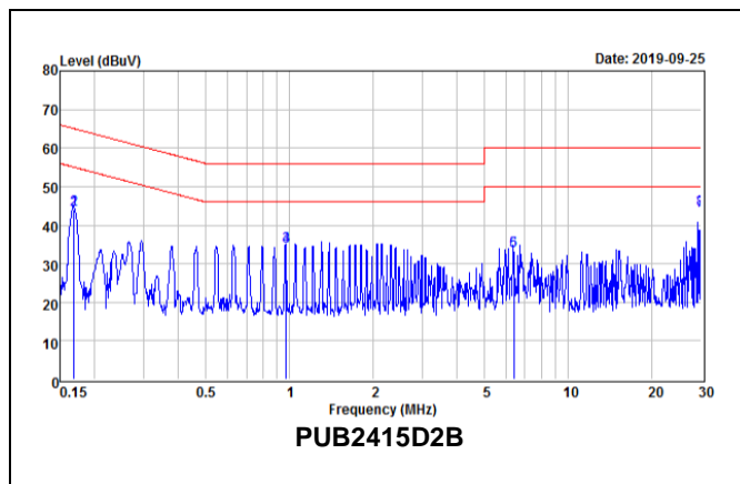
EMI with filter
