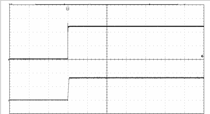
Start-up, enabled by connecting V_I at: T_{P1} = +25^\circ\text{C} , V_I = 24\text{ V} , V_O = 3.3\text{ V} I_O = 606\text{ mA} resistive load.
