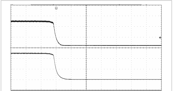
Shut-down, closed by disconnecting V_I at: T_{P1} = +25^\circ\text{C} , V_I = 5\text{ V} , V_O = 5\text{ V} I_O = 400\text{ mA} resistive load.
