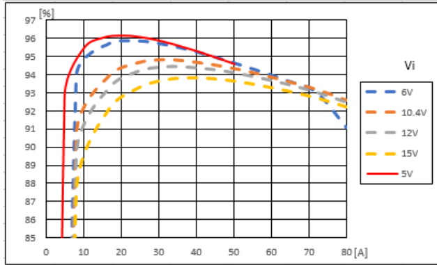
Driver losses excluded, 2 phases, fsw=800 kHz
