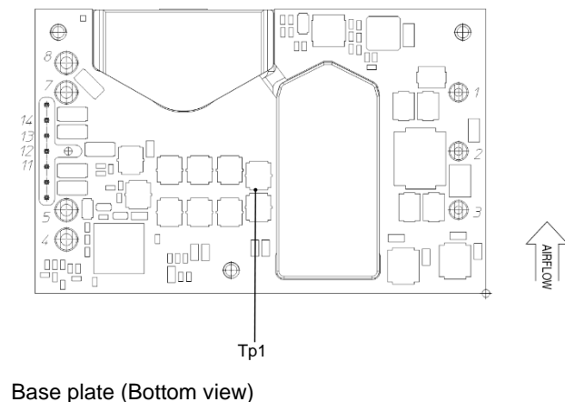
Base plate (Bottom view)
