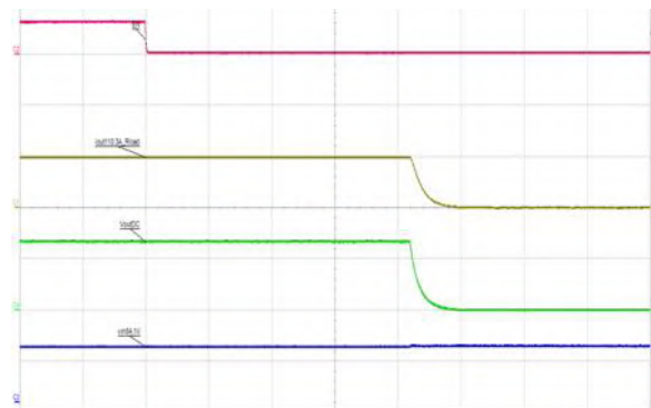
Output disabled by EN pin. V_{in} = 54\text{ V} , I_{out} = 100\text{ A} Scale from top: 5, 100, 5, 50 V/div, 500 \mu\text{s} /div.
