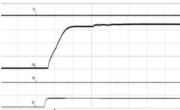
Output enabled by EN pin. V_{in} = 54\text{ V} , I_{out} = 0.3\text{ A} Scale from top: 50, 2, 5, 5 V/div, 2 ms/div.
