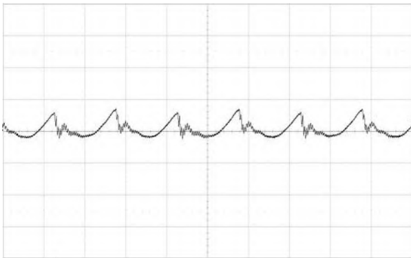
V_{in} = 54\text{ V} , I_{out} = 110\text{ A} , 20 MHz BW. Scale 10 mV/div, 0.5 \mu\text{s} /div.
