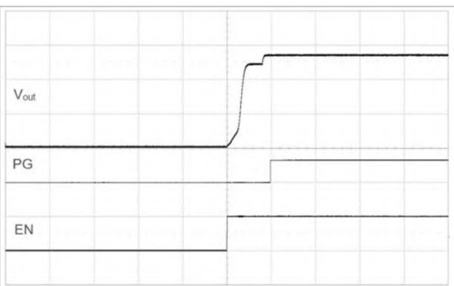
Output enabled by EN pin. V_{in} = 54\text{ V} , I_{out} = 1\text{ A} Scale from top: 5, 5, 5 V/div, 10 ms/div.
