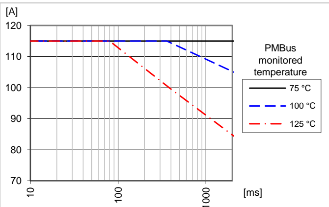
Max. peak output current vs pulse duration and PMBus monitored temperature when pulse starts. Initial Iout = 70 A. Simulated limit given by max. internal junction temperature (150 °C) of hotspot component. In practise, the max. peak current is also limited by the Timed OCP threshold and response time.
