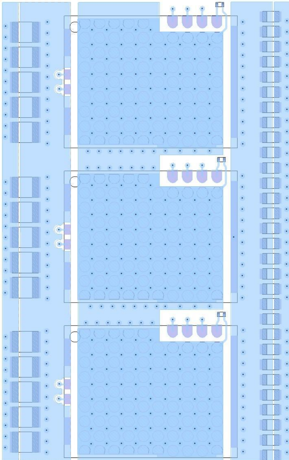
Layout for parallelling
