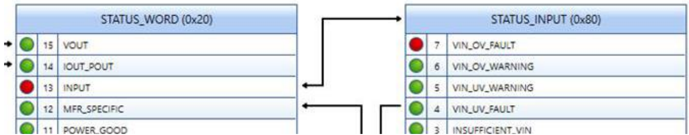
Picture 4: Detailed view - INPUT-VIN_OV_FAULT
