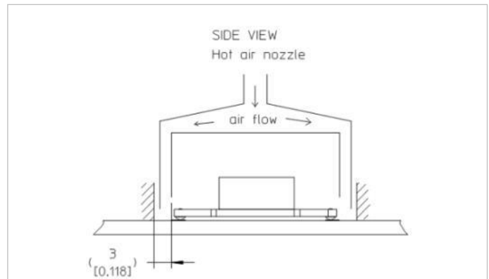
Figure 1: Schematic hot air nozzle design
