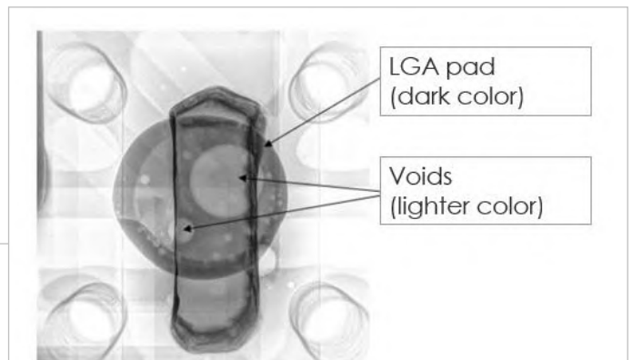
Picture 7: Close-up of the LGA pad with voids
