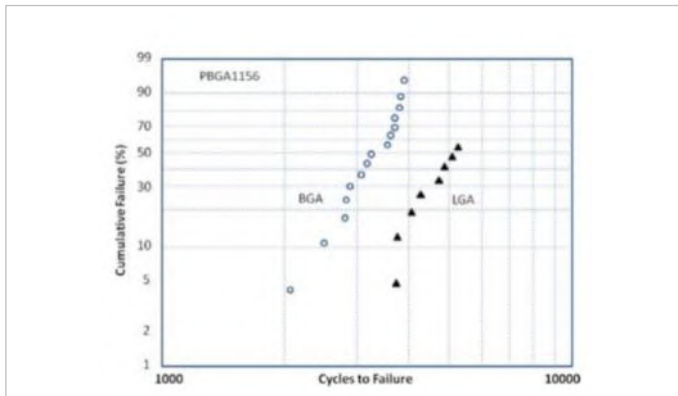
Picture 2: Weibull plot showing cycles to failure in -40°/125°C thermal cycling – SAC305 PBGA1156 and LGA 1156
