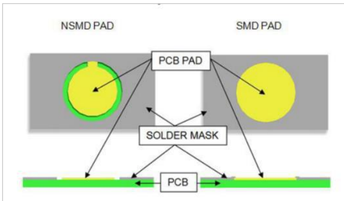
Picture 5: NSMD & SMD pad in comparison
