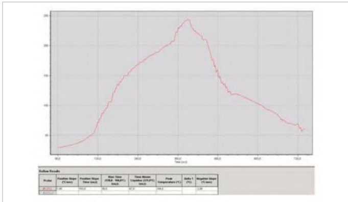
Picture 8: Reflow profile
