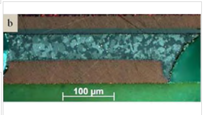
Picture 4: Cross polarized image of a 30 mil SAC305 LGA solder joint exhibiting an interlaced twinned grain structure
