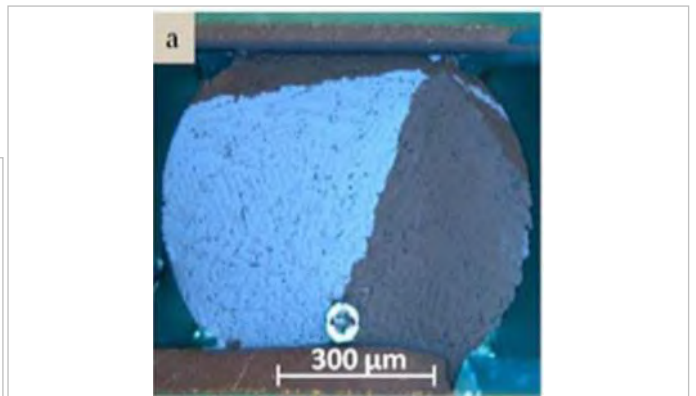
Picture 3: Cross polarized image of a 30 mil SAC305 BGA solder joint demonstrating the characteristic 'Beach Ball' microstructure.
