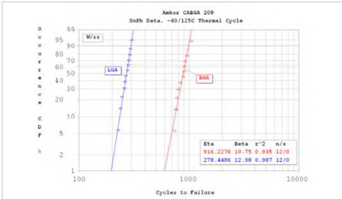
Picture 1: Weibull plot showing cycles to failure in -40°/125°C thermal cycling – Sn/Pb BGAs and corresponding LGAs
